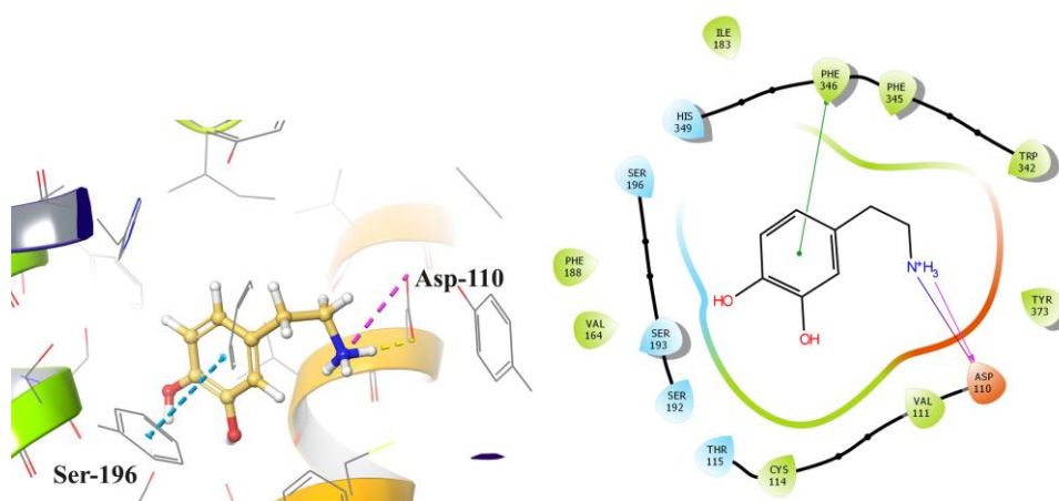
Figure: Dopamine docking with D3 (7CMV) receptor.
