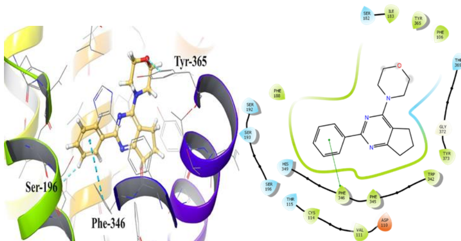
Figure: PP-43 docking with D3 (7CMV) receptor
