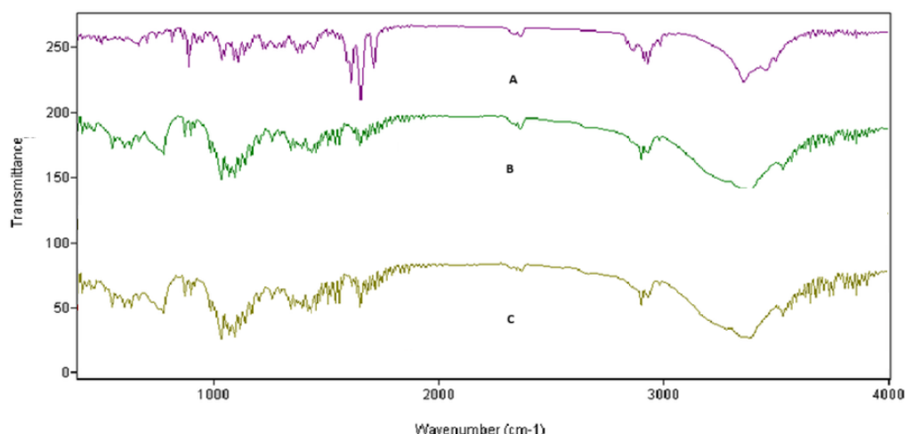
Figure 1. FTIR spectra of Prednisolone, AT-P and TF 3
