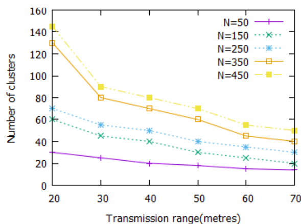
Figure 4 Transmission range against number of clusters
