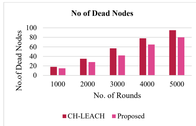
Figure 3: Comparison of Number of Dead Nodes
