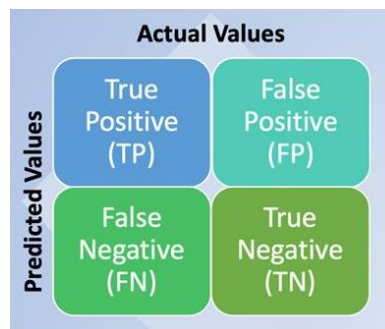
Figure 1: Confusion Matrix
